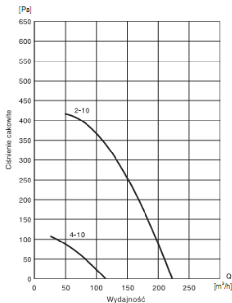
VASP 10
