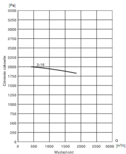
VASP 16
