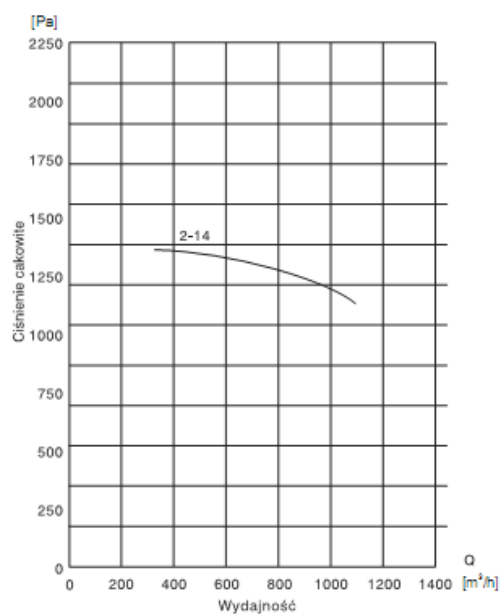
VASP 14
