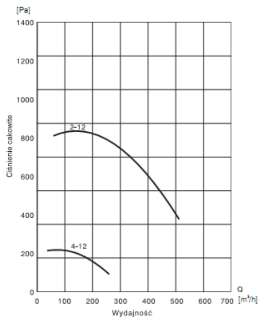
VASP 12
